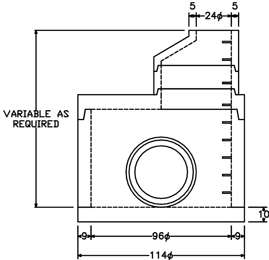
ELEVATION - ECCENTRIC
