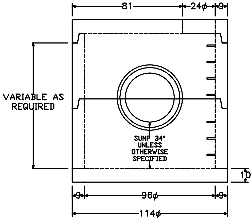
ELEVATION - ECCENTRIC
