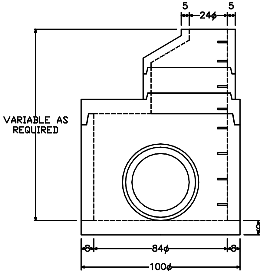
ELEVATION - ECCENTRIC
