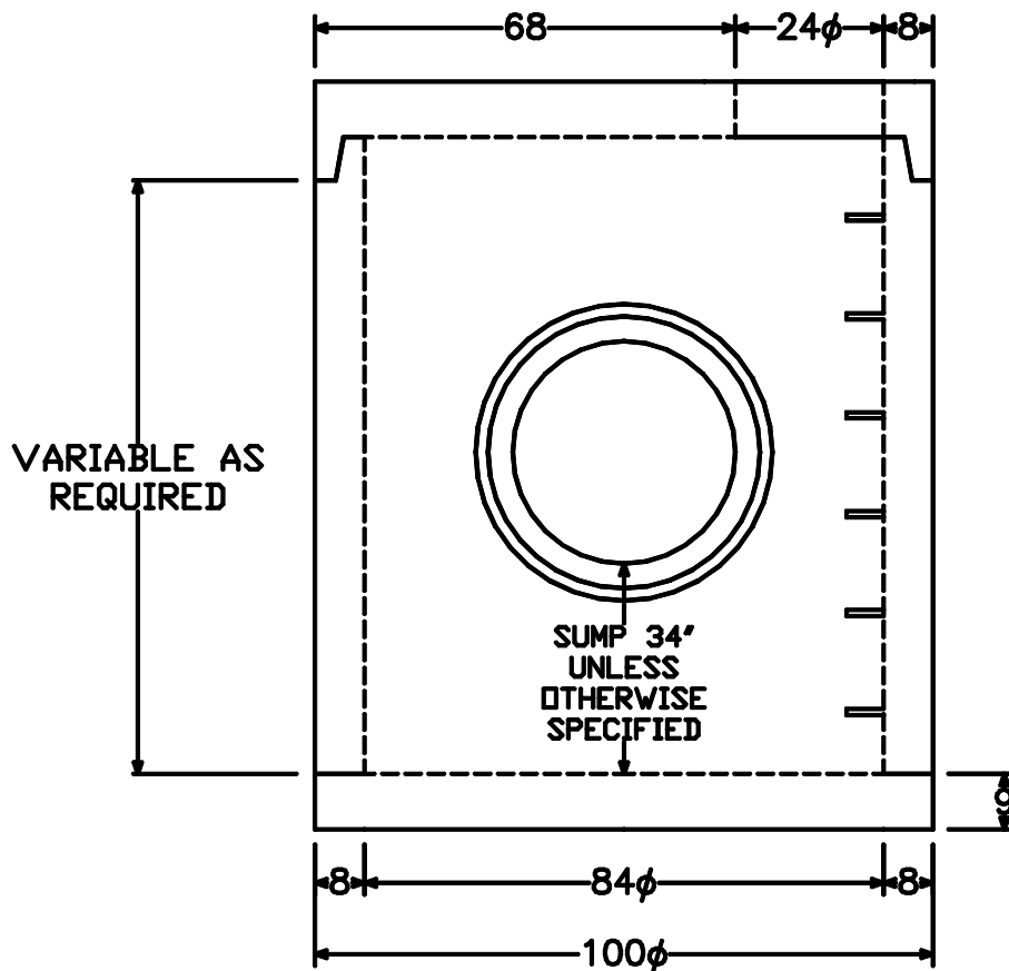
ELEVATION - ECCENTRIC
