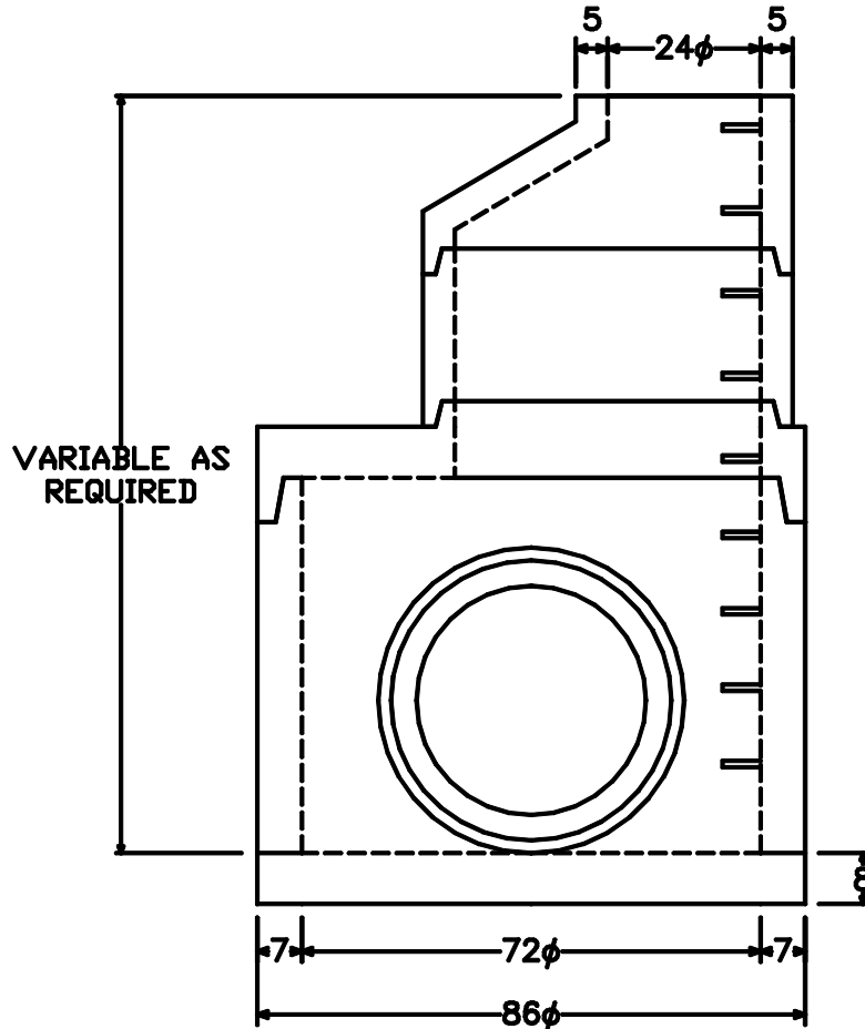
ELEVATION - ECCENTRIC
