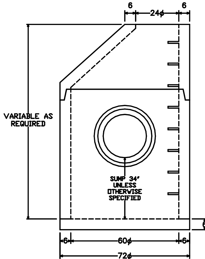
ELEVATION - ECCENTRIC
