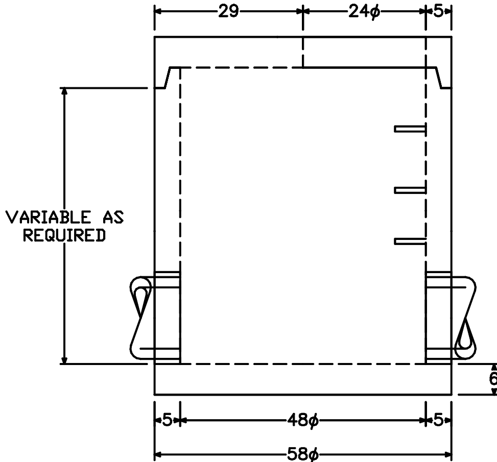
ELEVATION - ECCENTRIC
