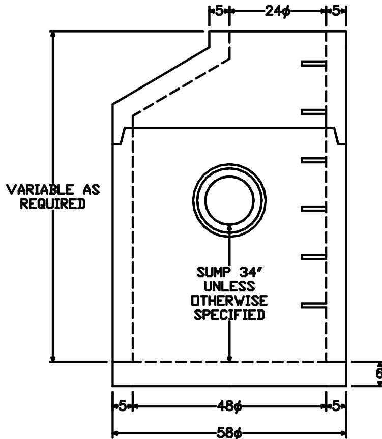
ELEVATION - ECCENTRIC
