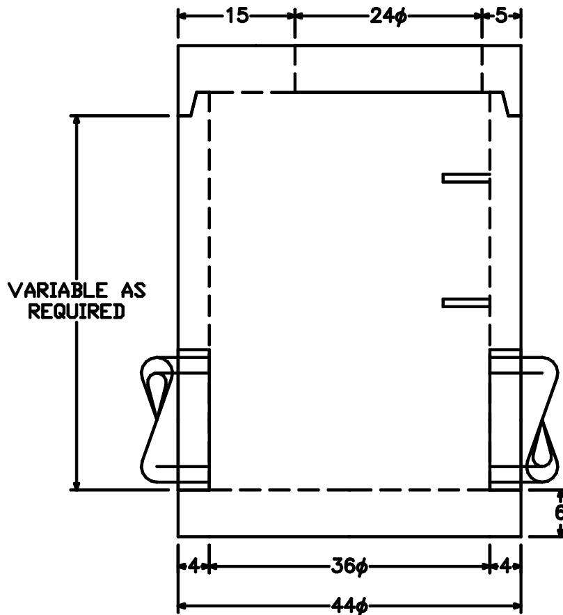
ELEVATION - ECCENTRIC
