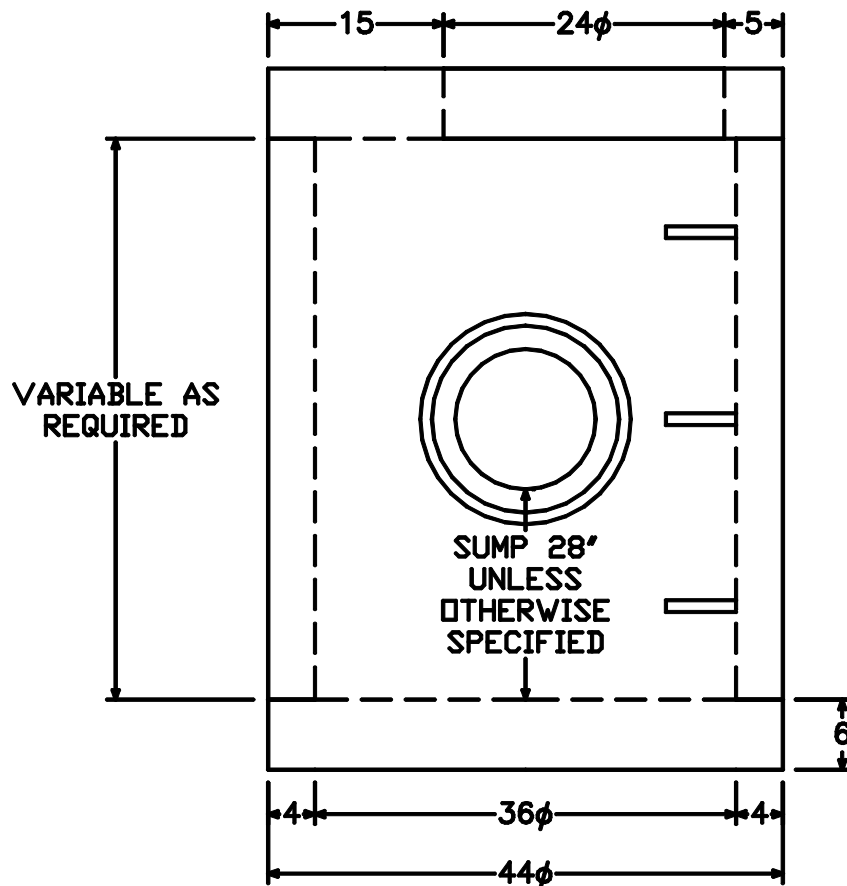
ELEVATION - ECCENTRIC
