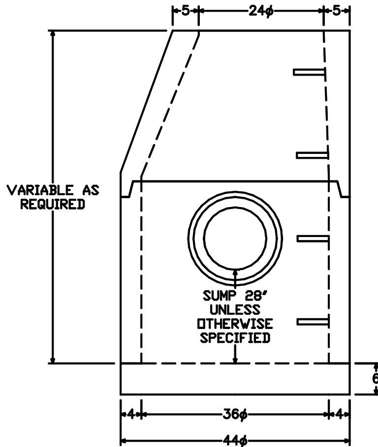
ELEVATION - ECCENTRIC
